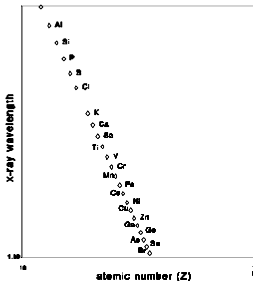
Figure 1-4 Moseley's law
